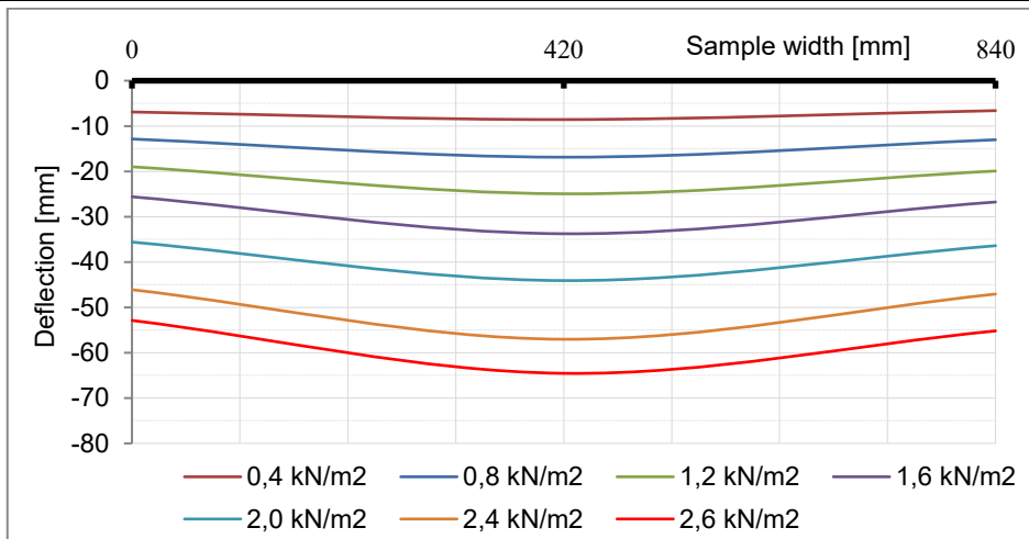
Figure 8. Mid-span cross-section deflection diagram, source: Authors
